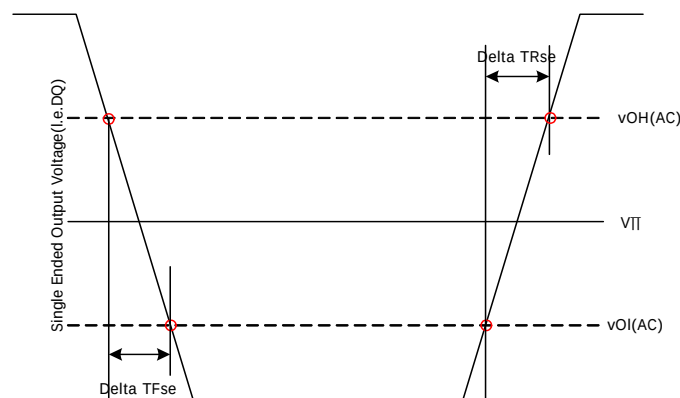
Single Ended Output Slew Rate Definition
