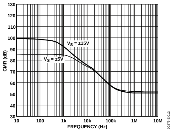
Figure 15. Common-Mode Rejection vs. Frequency
