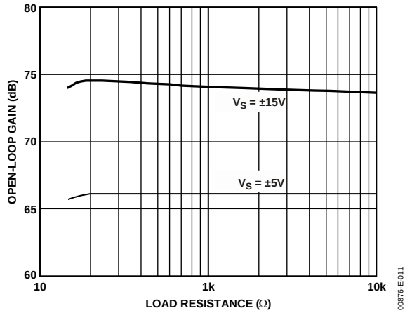
Figure 13. Open-Loop Gain vs. Load Resistance
