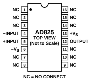
Figure 5. 16-Lead SOIC
