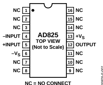
Figure 2. 16-Lead Plastic SOIC (RW-16) Package
