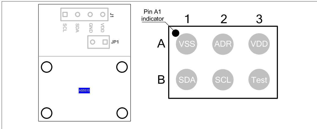
Figure 3. Pin Configuration of AS5510 (Top View)
