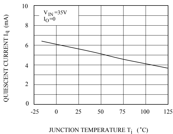
Fig.7 T_j - I_q
