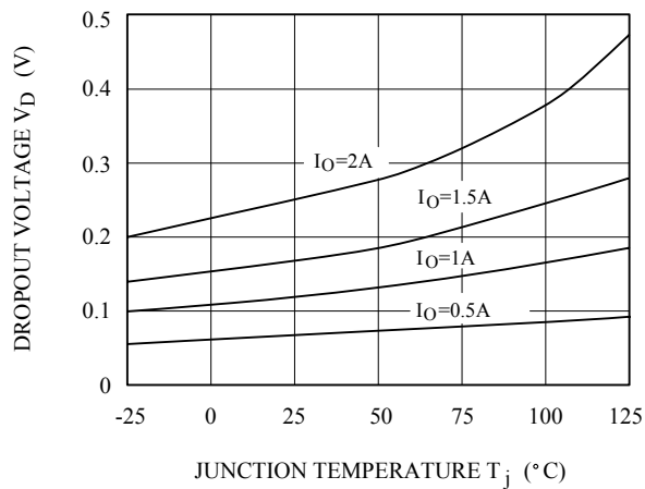
Fig.6 T_j - V_D
