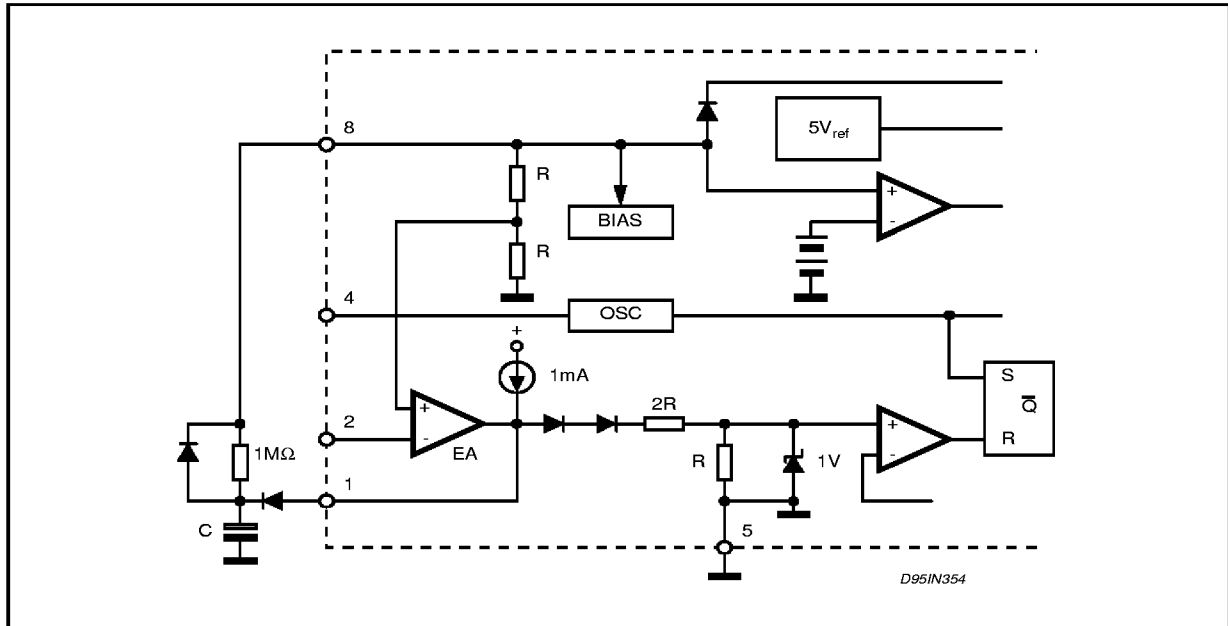
Figure 23: Soft-Start Circuit
