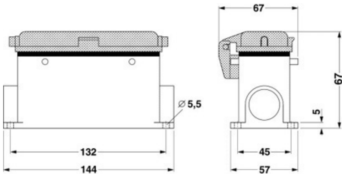
Dimensioned drawing
