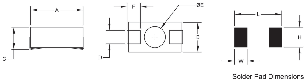
Solder Pad Dimensions
