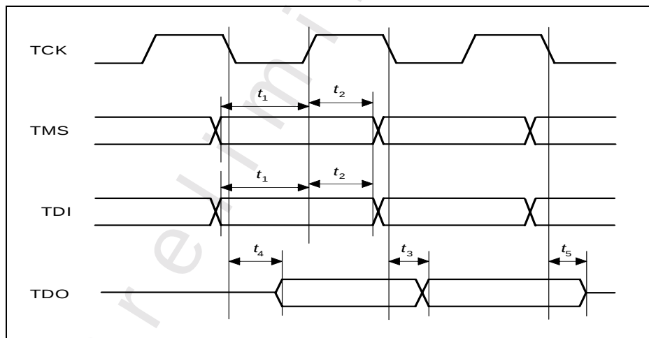
Figure 45 JTAG Timing
