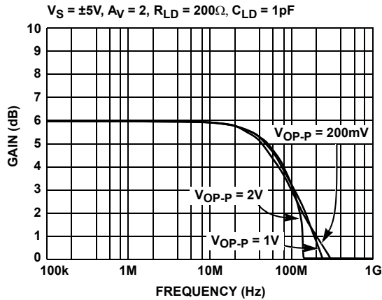
FIGURE 1. FREQUENCY RESPONSE
