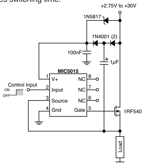
Figure 3. Bootstrapped Hgh-Side Driver
