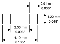
Outline SOD123
