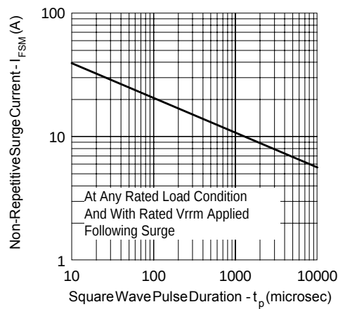
Fig. 7 - Maximum Non-Repitive Surge Current
