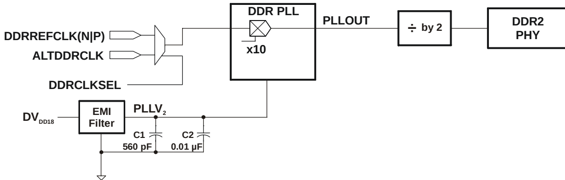
Figure 8-14 PLL2 Block Diagram
