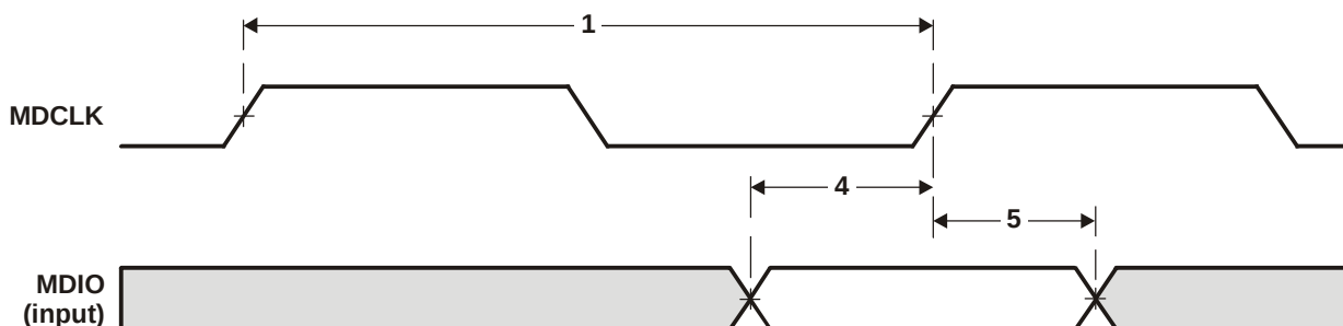
Figure 8-43 MDIO Input Timing
