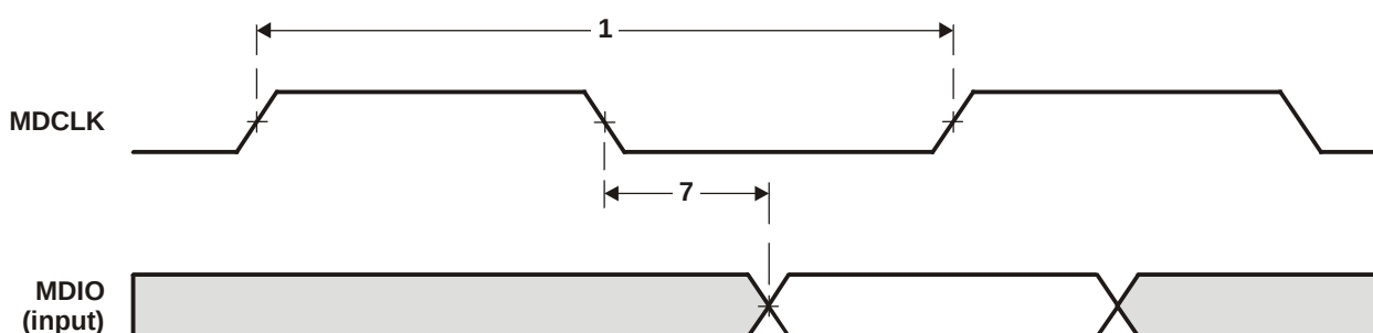
Figure 8-44 MDIO Output Timing
