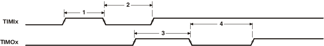
Figure 8-45 Timer Timing
