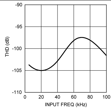
Figure 24. THD vs. INPUT Frequency
