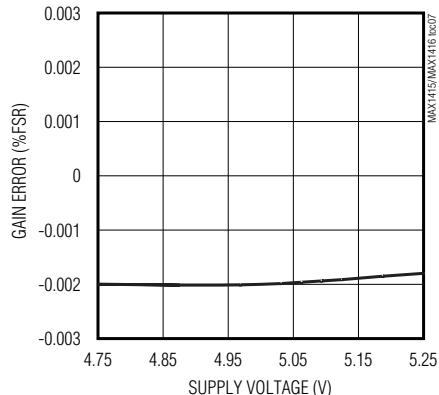
GAIN ERROR vs. SUPPLY VOLTAGE (MAX1416)
