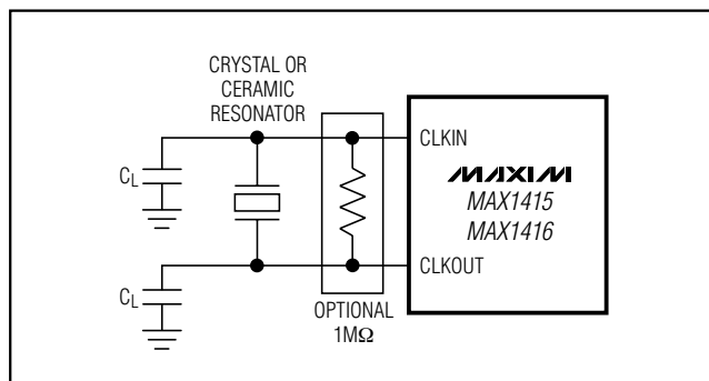
Figure 7. Using a Crystal or Ceramic Oscillator
