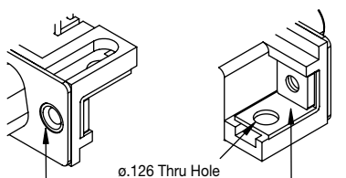
#4-40 Threaded Insert
