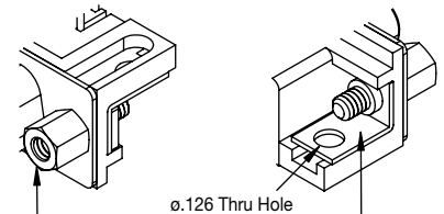
#4-40 Threaded Insert with Removable Jackscrew
