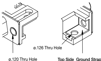
ø.120 Thru Hole
