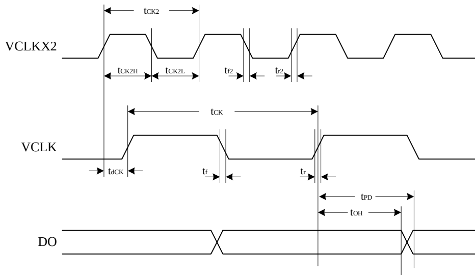
AL700/701/710 601 16-bit Output Timing
