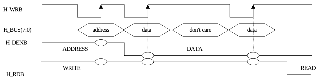
Figure 6: Host Write Cycle
