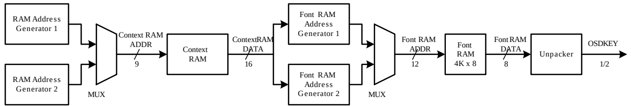
Figure 14: The Addressing of Context and Font RAMs
