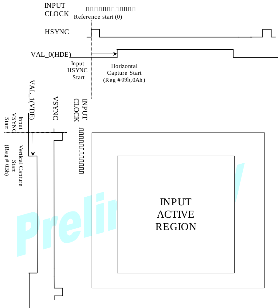
Figure 1: Input Video Timing
