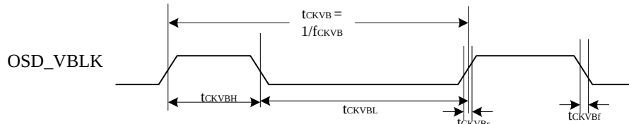
OSD Video Blank Control Timing
