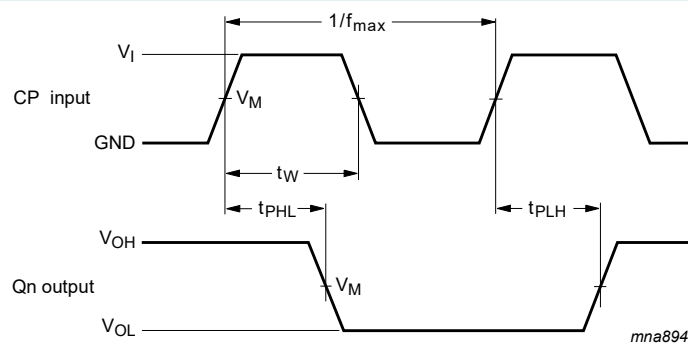
Fig. 5. Clock (CP) to output (Qn) propagation delays, the clock pulse width and the maximum frequency
