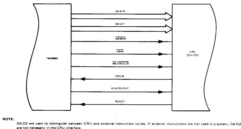
FIGURE 18 – TMS9995 CRU INTERFACE
