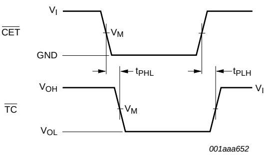
Measurement points are given in Table 8 . Logic levels: V_{OL} and V_{OH} are the typical output voltage levels that occur with the output load.
