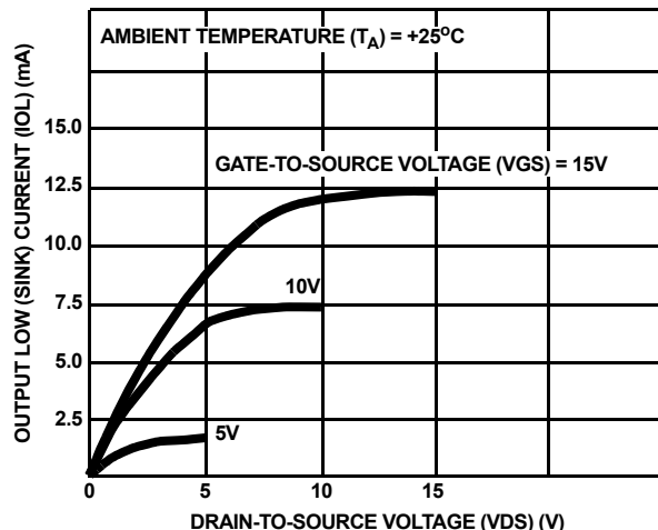
FIGURE 2. MINIMUM N OUTPUT LOW (SINK) CURRENT CHARACTERISTICS
