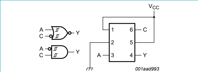
Fig. 8. 2-input AND gate with input A inverted or 2-input NOR gate with inverted C input
