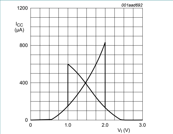
Fig. 18. Typical transfer characteristics; V CC = 3.0 V
