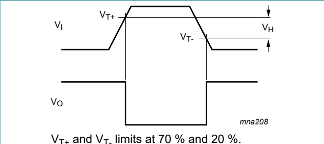
Fig. 16. Definition of V T+ , V T- and V H
