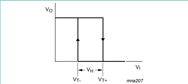
Fig. 15. Transfer characteristic
