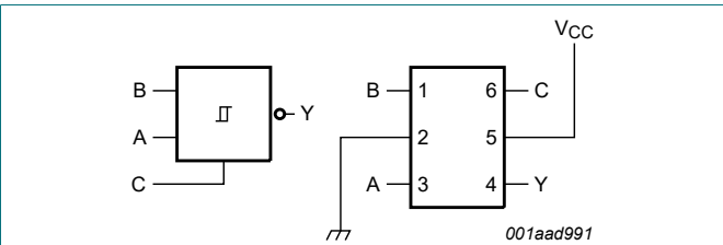
Fig. 6. 2-input MUX with inverted output
