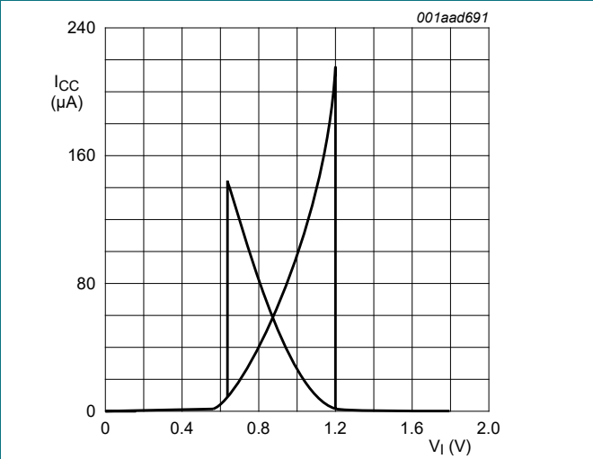
Fig. 17. Typical transfer characteristics; V CC = 1.8 V
