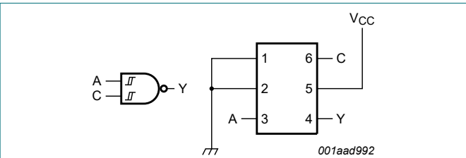
Fig. 7. 2-input NAND gate
