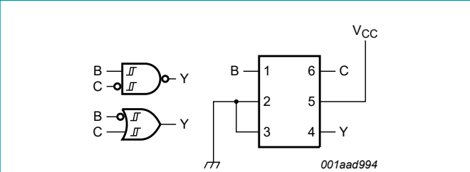
Fig. 9. 2-input OR gate with input B inverted or 2-input NAND gate with input C inverted
