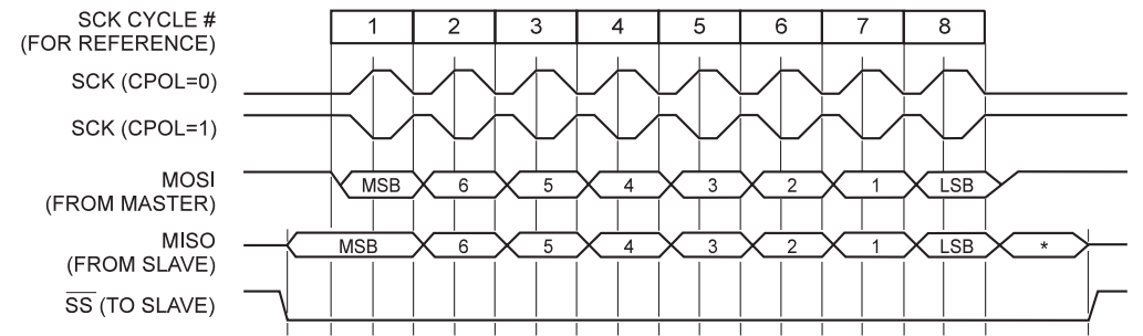
Figure 42. SPI Transfer Format with CPHA = 0 and DORD = 0
