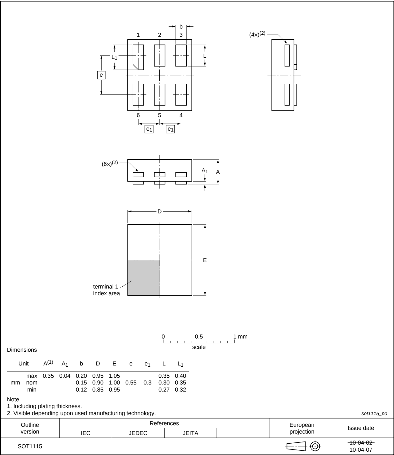
Fig 18. Package outline SOT1115 (XSON6) 74CBTLV1G125 All information provided in this document is subject to legal disclaimers. © NXP B.V. 2012. All rights reserved. Product data sheet Rev. 4 — 5 September 2012 16 of 21
