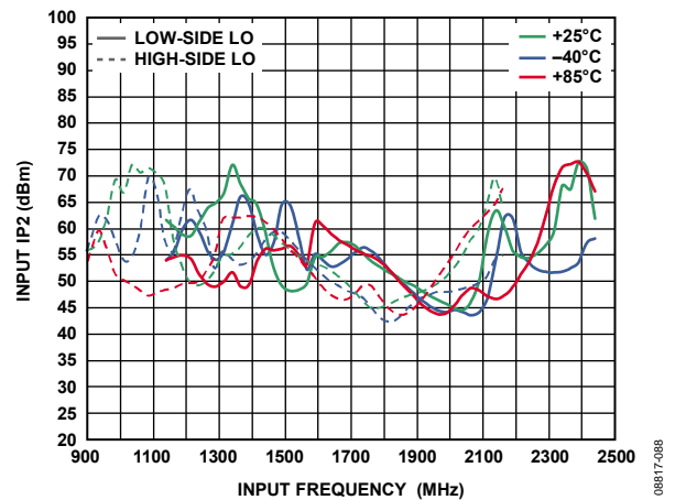
Figure 8. Input IP2 vs. Input Frequency
