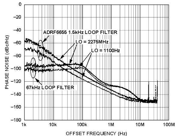
Figure 68. Phase Noise with Different Loop Filters
