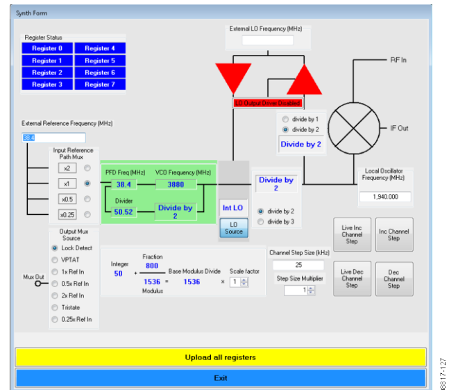
Figure 67. ADRF6655 Synthesizer Settings User Interface
