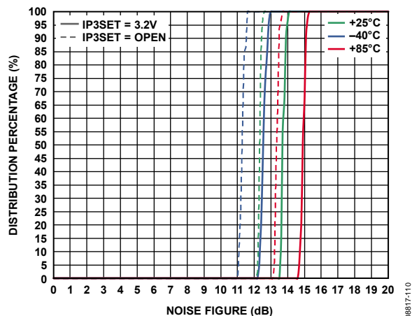
Figure 41. Rx Noise Figure CCDF
