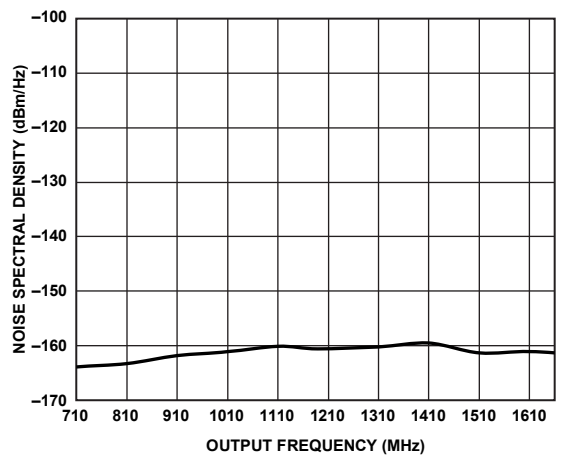
Figure 21. Output Noise Spectral Density vs. Output Frequency
