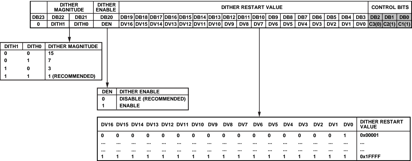
Figure 73. Σ-Δ Modulator Dither Control Register (R3)
