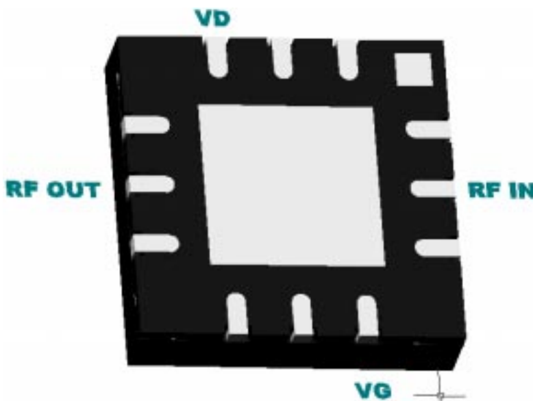
Bottom View
