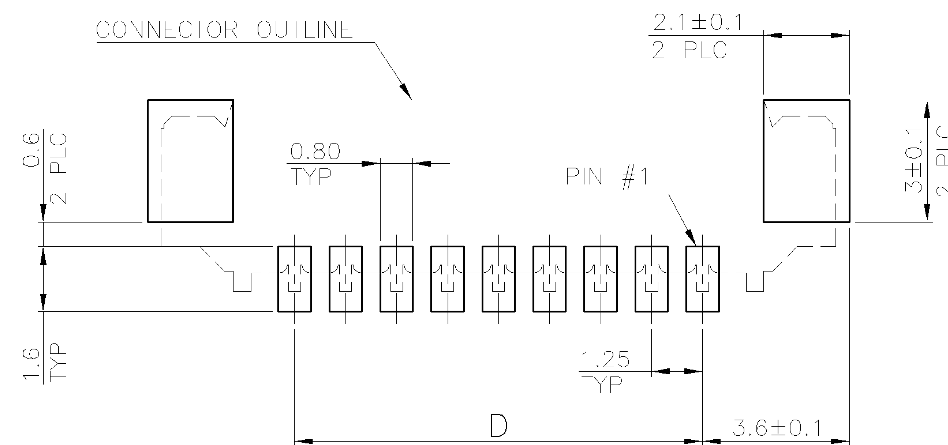
RECOMMENDED PC BOARD LAYOUT (TOLERANCE: \pm 0.05 )
