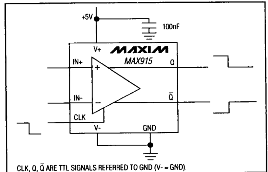
Figure 3. Single-Supply Operation
