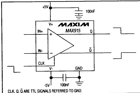
Figure 2. Dual-Supply Operation
