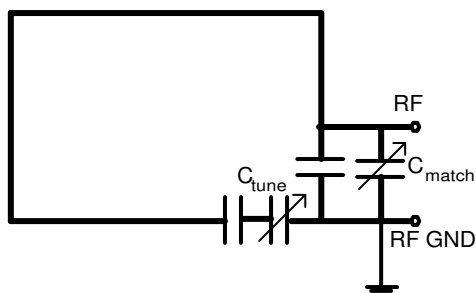
Loop antenna
