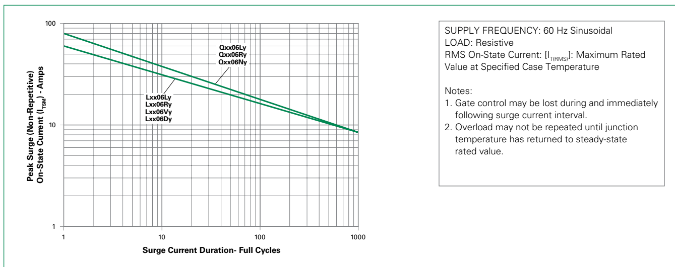
Figure 12: Surge Peak On-State Current vs. Number of Cycles (Sensitive / Standard Triac)
