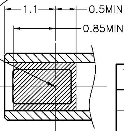
SECT. E-E (SCALE 20:1)
