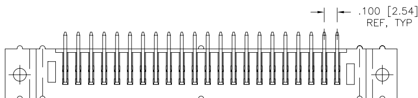
VIEW Y-Y
