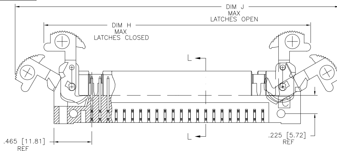
VIEW Y-Y
