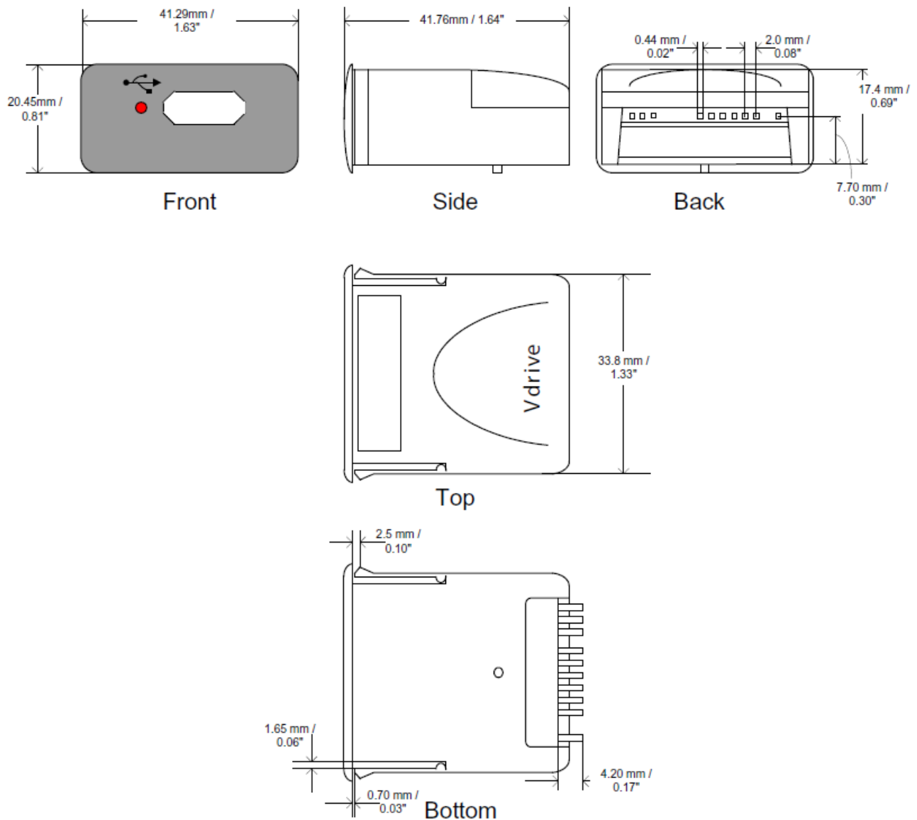
Figure 8.1 – VDrive3 Dimensions
