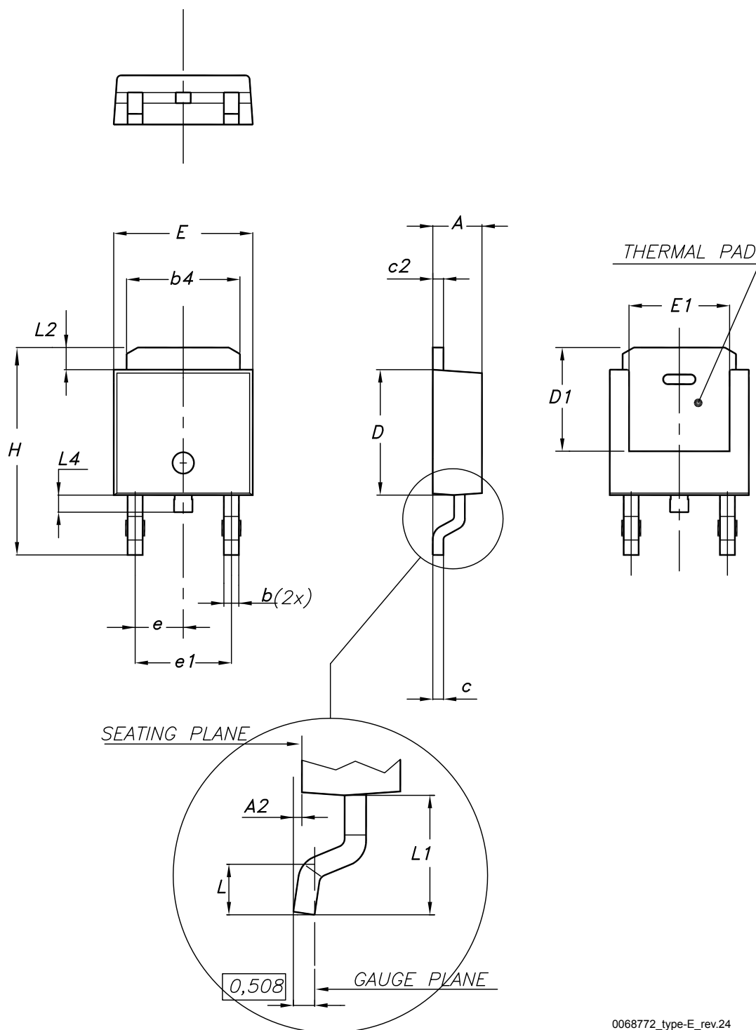
Figure 18. DPAK (TO-252) type E package outline
