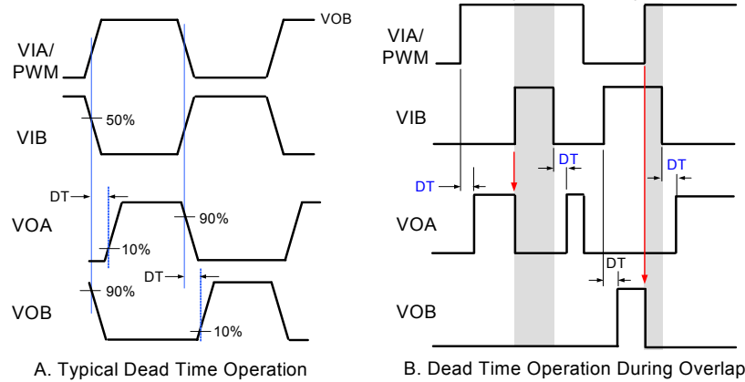
Figure 41. Dead Time Waveforms for High-Side/Low-Side Two-Input Drivers
