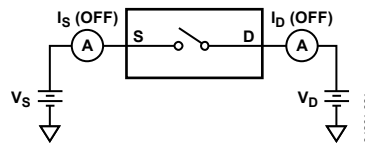
Figure 27. Off Leakage
