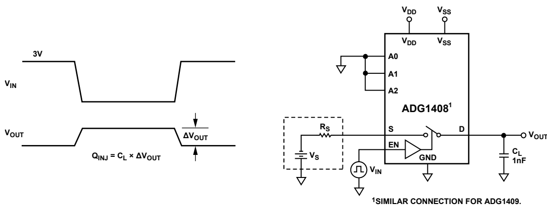
Figure 32. Charge Injection
