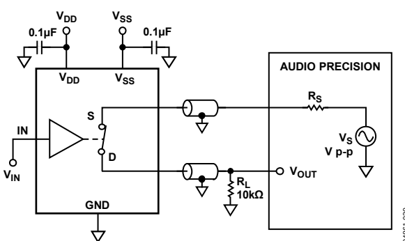
Figure 36. THD + Noise
