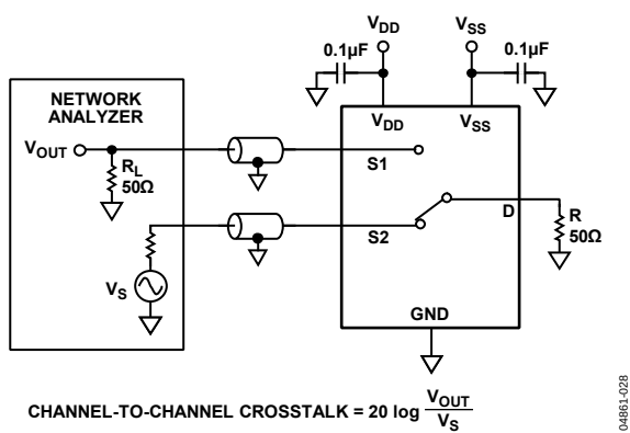
Figure 34. Channel-to-Channel Crosstalk
