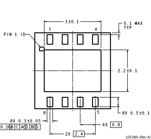
8-Lead LLP NS Package Number LDC08A
