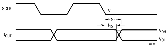
Figure 21. SCLK to DOUT Delay
