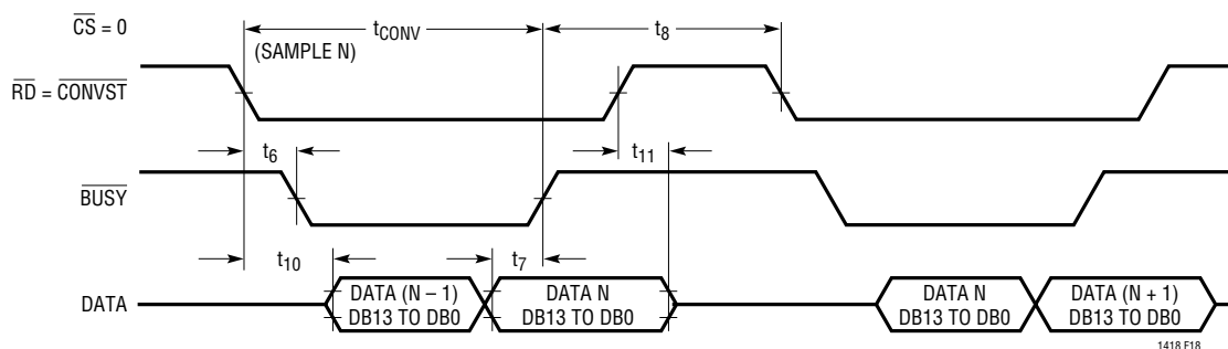
Figure 18. Slow Memory Mode Timing
