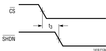
Figure 13b. \overline{\text{CS}} to \overline{\text{SHDN}} Timing
