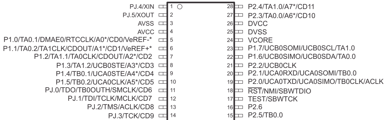
Figure 4-5. 28-Pin PW Package
