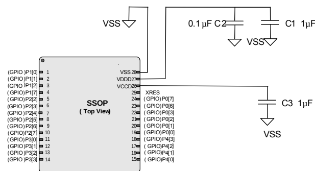
Figure 11. 28-SSOP Example
