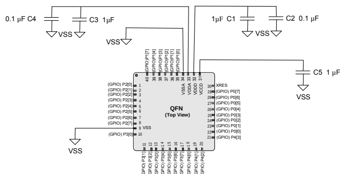
Figure 10. 40-pin QFN Example
