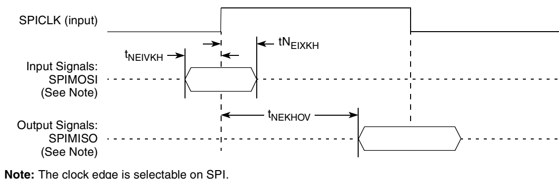
Figure 46. SPI AC Timing in Slave Mode (External Clock) Diagram
