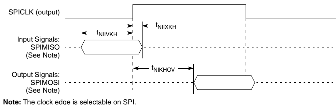
Figure 47. SPI AC Timing in Master Mode (Internal Clock) Diagram
