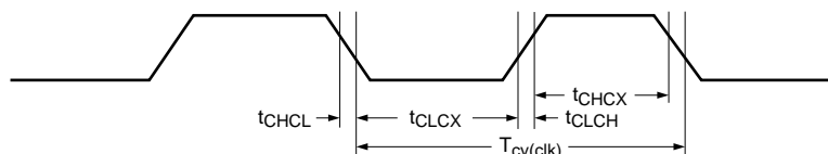
Fig 20. External clock timing (with an amplitude of at least V_{i(RMS)} = 200\text{ mV} )
