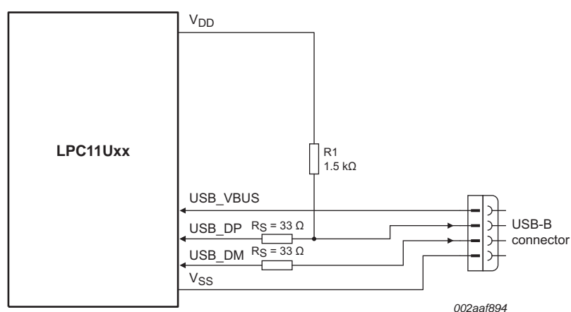
Fig 26. USB interface on a bus-powered device
