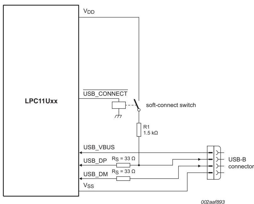
Fig 28. USB interface with soft-connect
