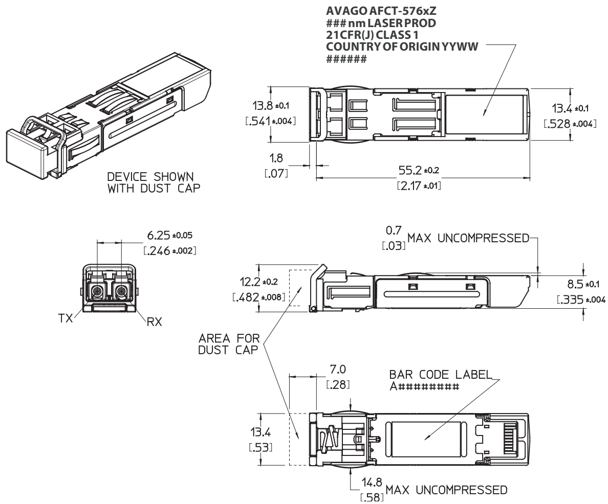
Figure 6. Module Drawing
