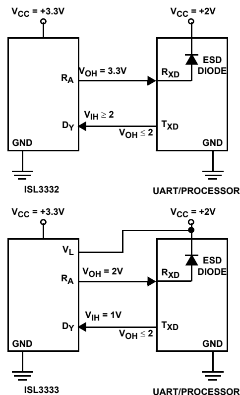
FIGURE 12. USING V L PIN TO ADJUST LOGIC LEVELS
