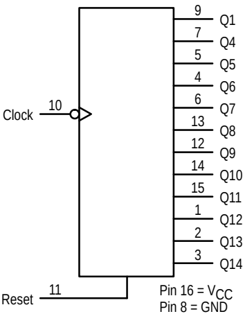
LOGIC DIAGRAM
