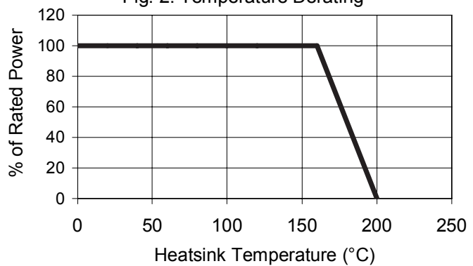
Fig. 2: Temperature Derating
