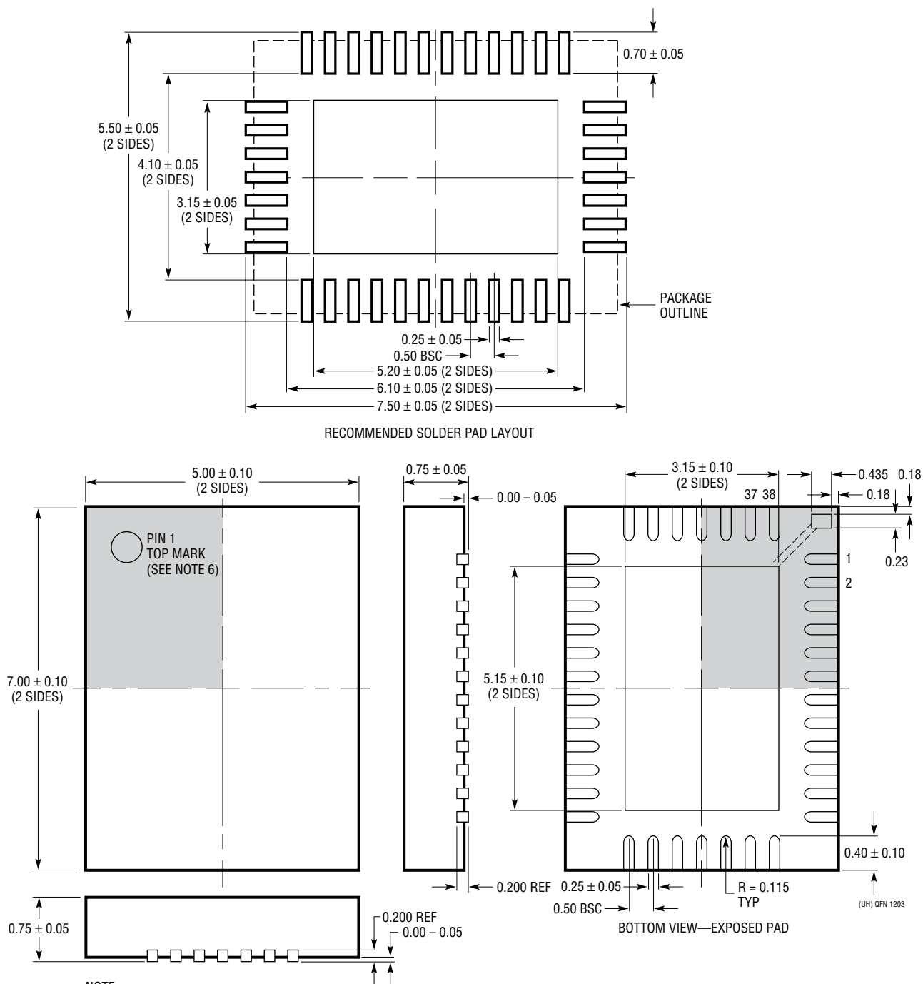
UHF Package 38-Lead Plastic QFN (5mm × 7mm) (Reference LTC DWG # 05-08-1701)
