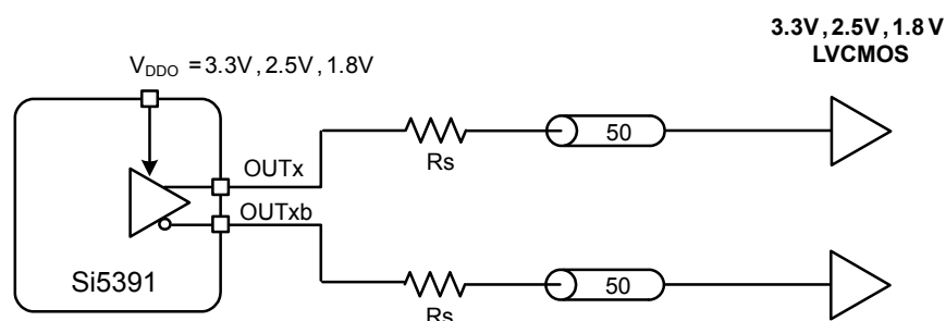
Figure 4.7. LVCMOS Output Terminations
