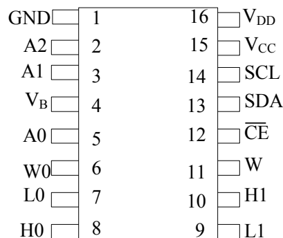
16-Pin SOIC (150-mil)
