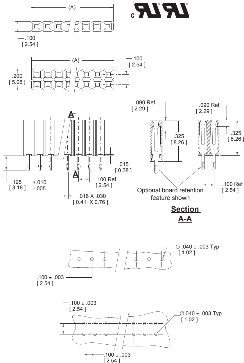
Recommended Mounting Hole Patterns (Shown for Mounting Side of Board)
