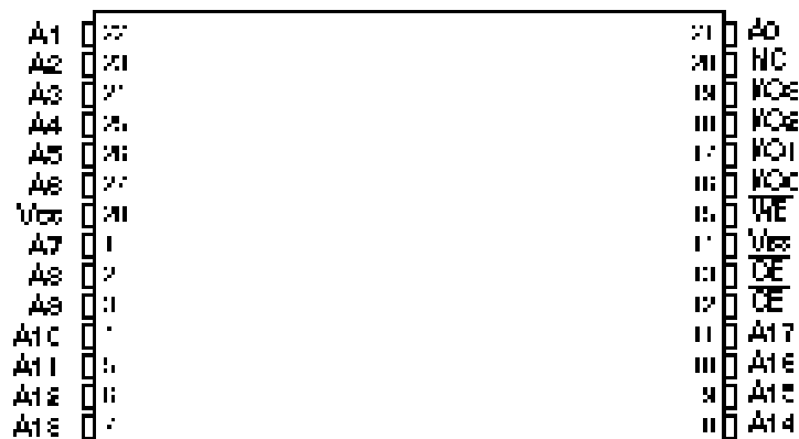
TSOP
